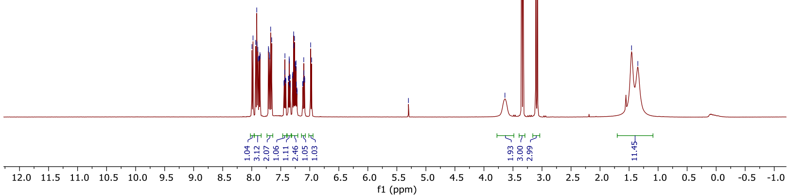
^1\text{H} NMR spectrum of ( R )-cat ( \text{CDCl}_3 )
